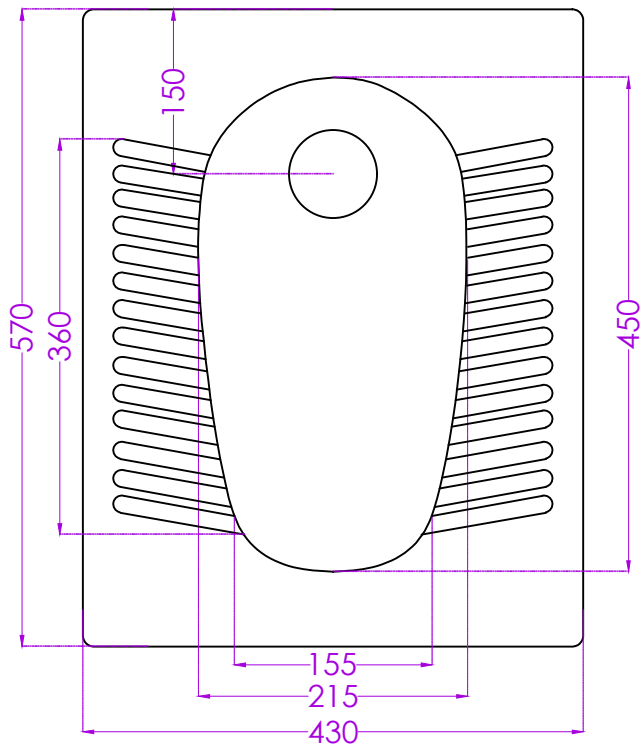
PLAN
