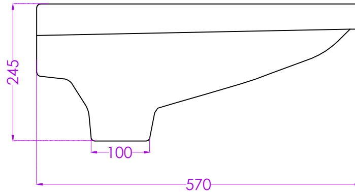
SIDE
